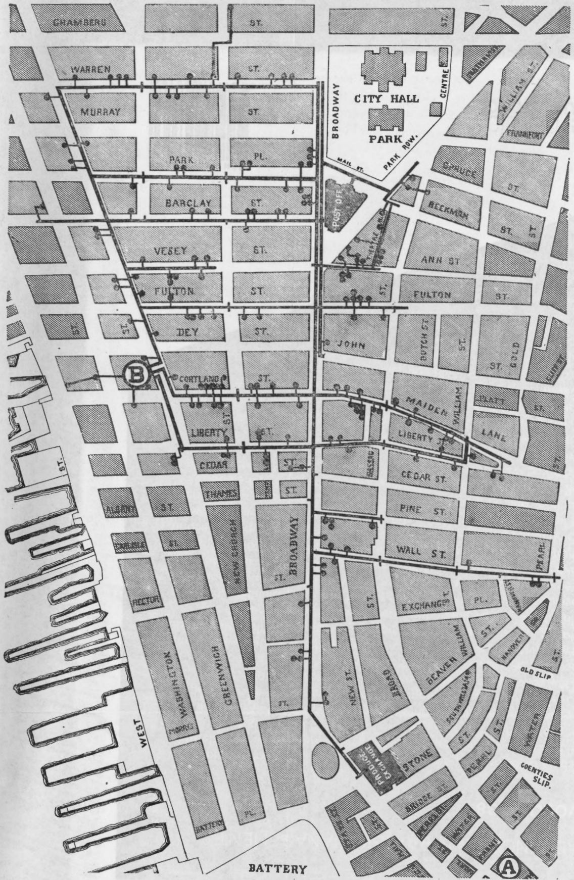
Map showing the location of the Mains and Services of the New York Steam Co.
