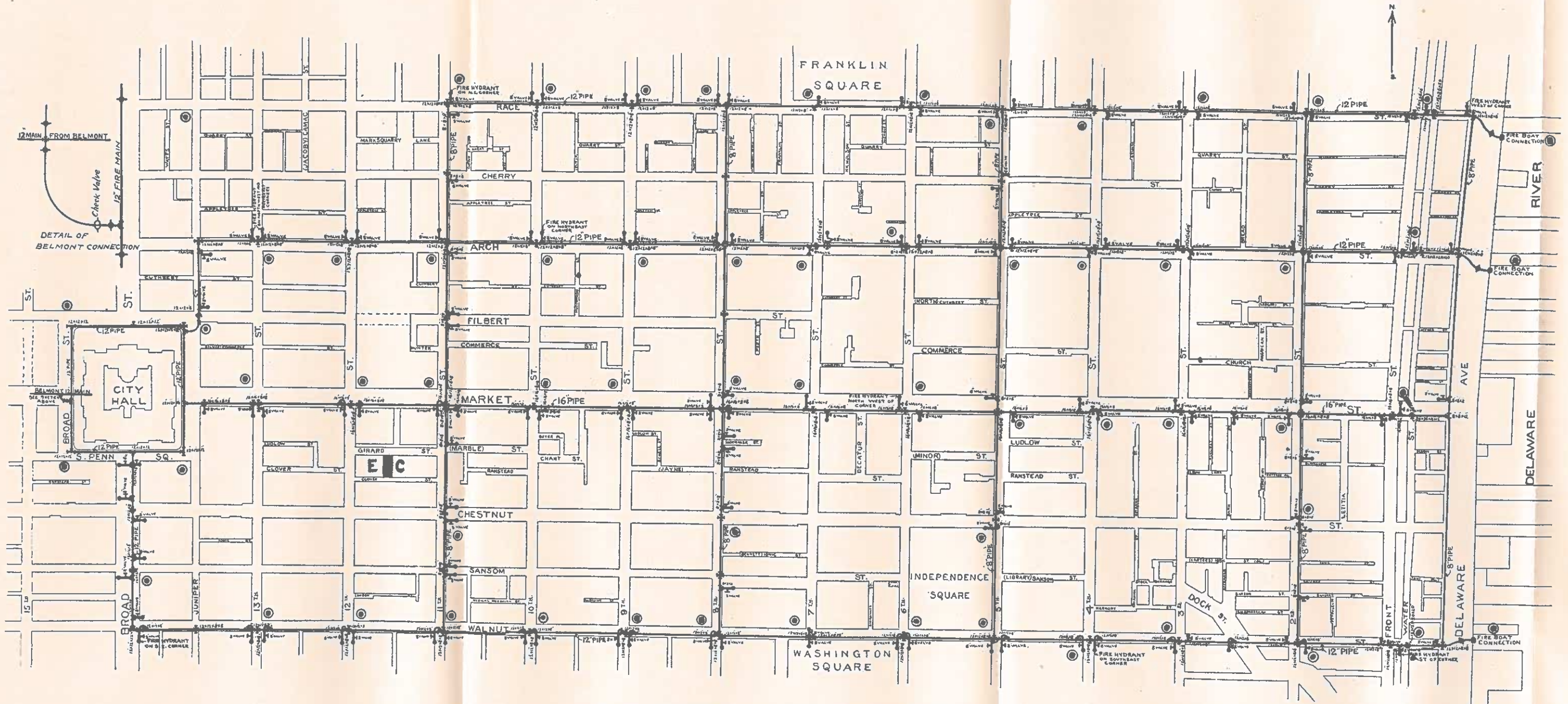
PLAN OF PHILADELPHIA FIRE MAIN SYSTEM. SCALE, 1 INCH = 484 FEET.
